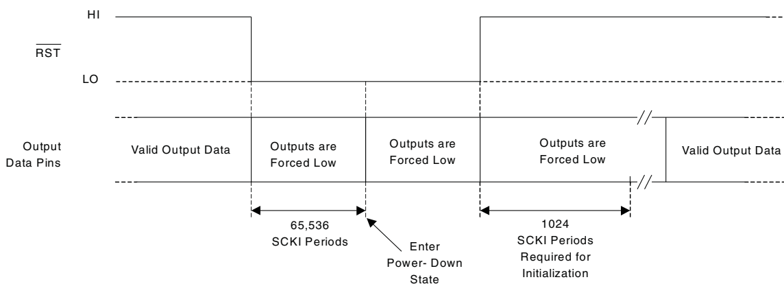
Figure 11. ADC Digital Output State for Power-Down Operations
