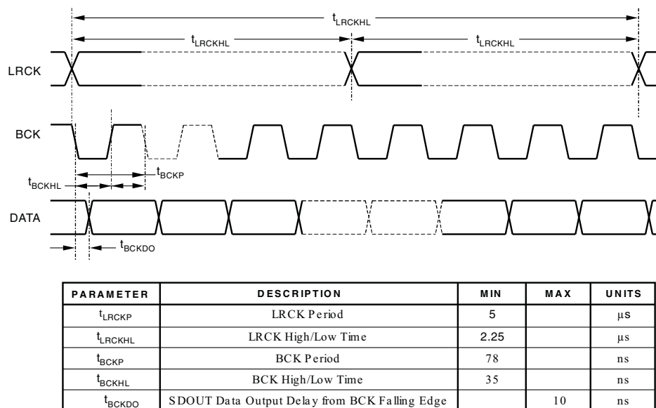
Figure 6. Master and Slave Mode Audio Serial Port Timing: Left Justified, Right Justified, and Philips I 2 S
